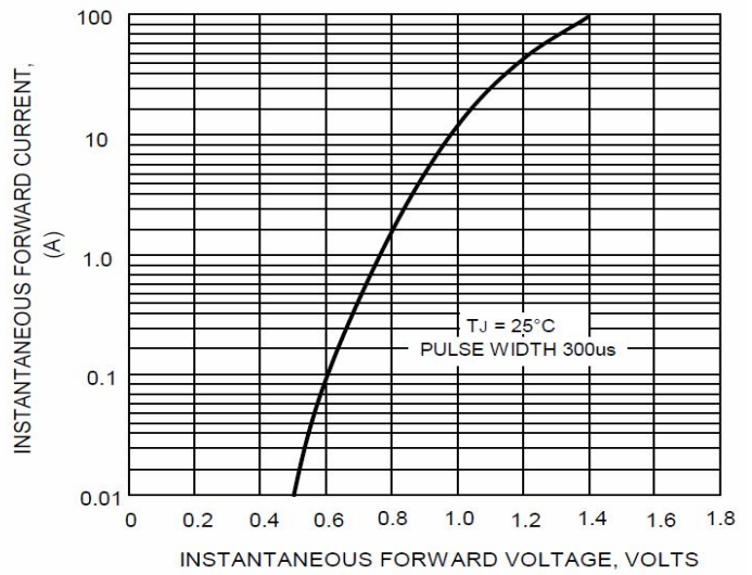
FIG.4-TYPICAL FORWARD CHARACTERISTICS
