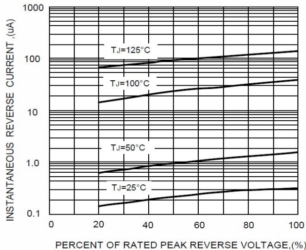
FIG.5-TYPICAL REVERSE CHARACTERISTICS
